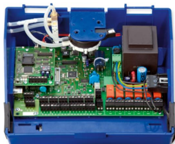
EASYLAB-REGULATOR TCU3
