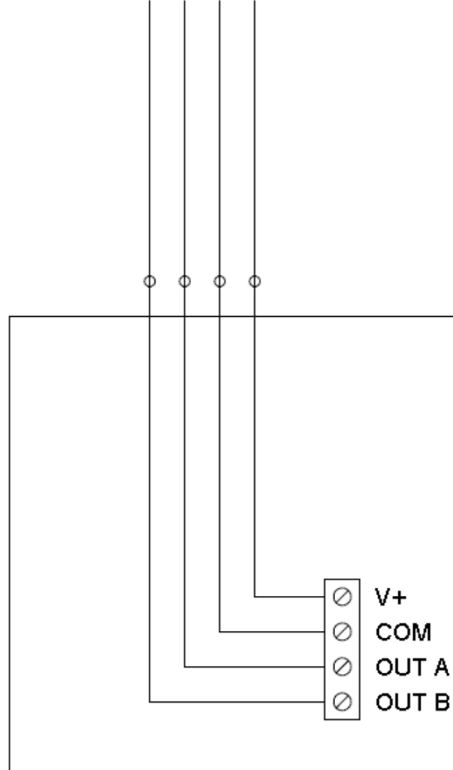
OptoSense IAQ Sensor
