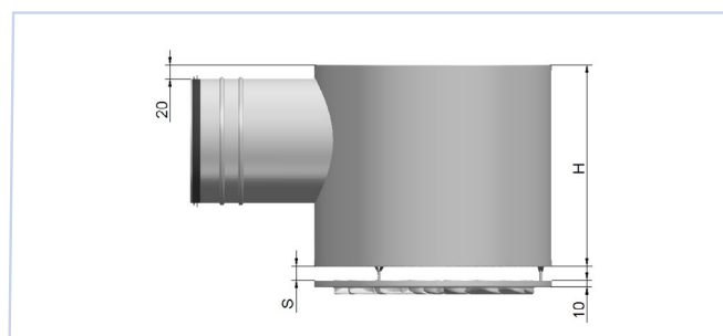
Figur 1, Tellus-Opus-L
