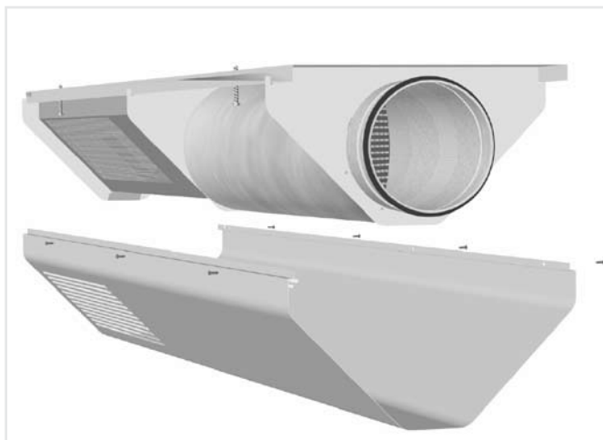
Fig. 7: Installation
