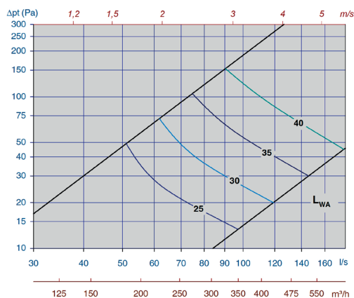
Diagram 19, Tellus-D-Opus-200-min. slot height
