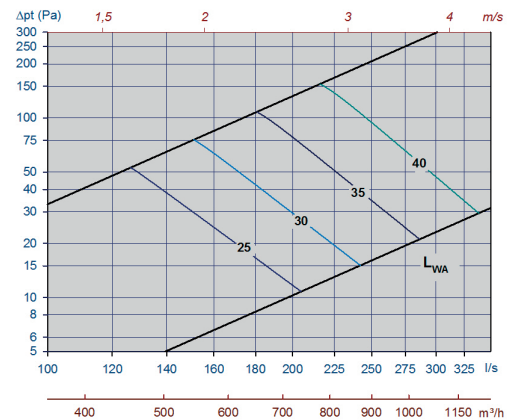
Diagram 18, Tellus-Opus-315-max. slot height
