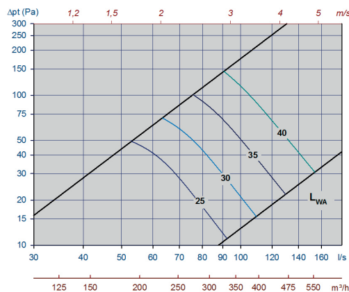
Diagram 11, Tellus-Opus-200-mid. slot height
