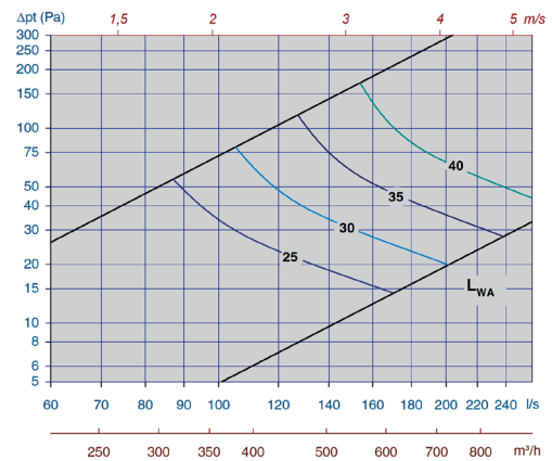
Diagram 24, Tellus-D-Opus-250-max. slot height
