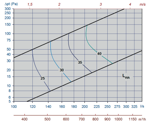
Diagram 16, Tellus-Opus-315-min. slot height
