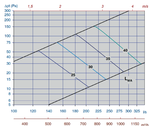
Diagram 26, Tellus-D-Opus-315-mid. slot height
