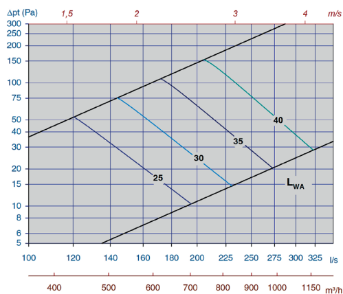
Diagram 25, Tellus-D-Opus-315-min. slot height
