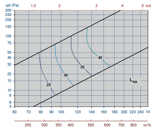
Diagram 13, Tellus-Opus-250-min. slot height.
