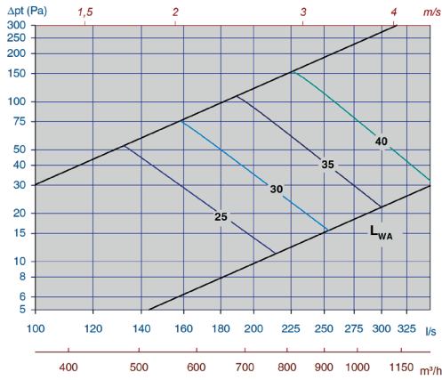
Diagram 27, Tellus-D-Opus-315-max. slot height
