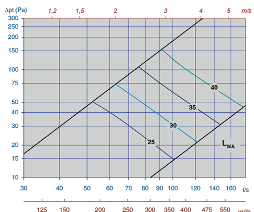
Diagram 20, Tellus-D-Opus-200- mid. slot height
