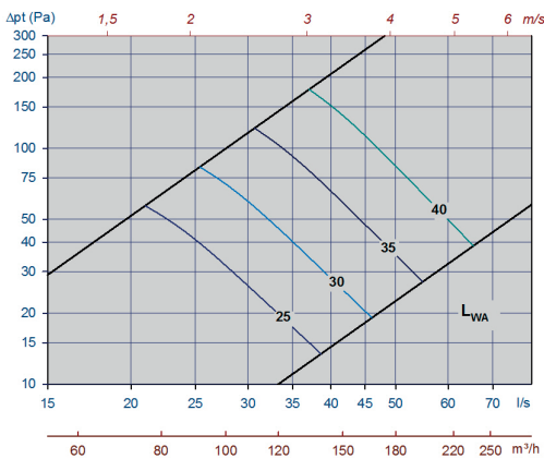
Diagram 5, Tellus-Opus-125-mid. slot height
