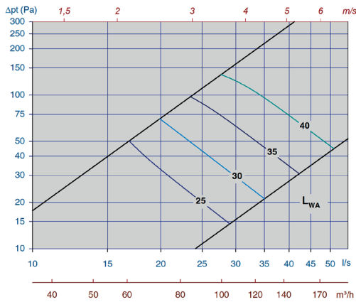
Diagram 3, Tellus-Opus-100-max. slot height
