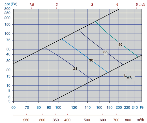
Diagram 22, Tellus-D-Opus-250-min. slot height
