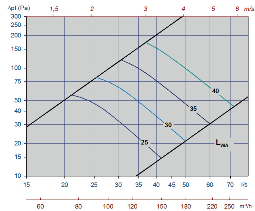
Diagram 6, Tellus-Opus-125-max. slot height
