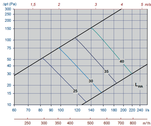
Diagram 15, Tellus-Opus-250-max. slot height
