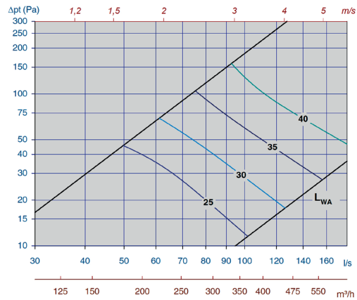
Diagram 21, Tellus-D-Opus-200-max. slot height
