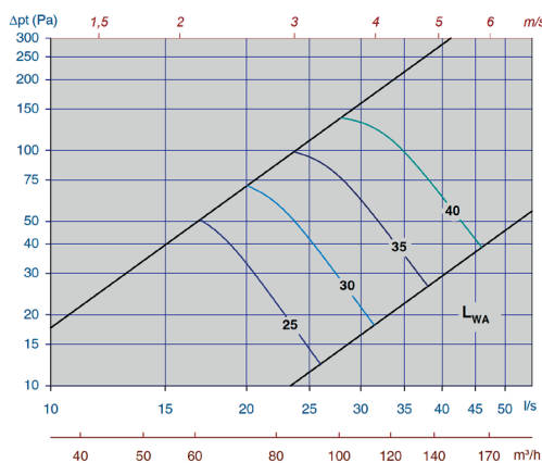
Diagram 1, Tellus-Opus-100-min. slot height
