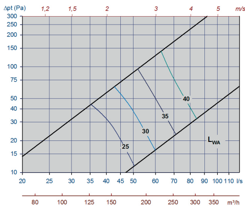
Diagram 7, Tellus-Opus-160-min. slot height
