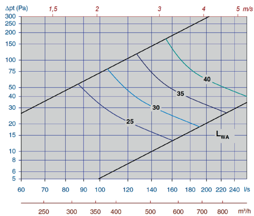
Diagram 23, Tellus-D-Opus-250-mid. slot height
