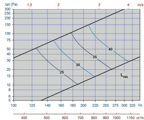
Diagram 17, Tellus-Opus-315-mid. slot height
