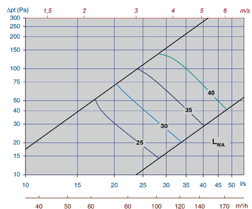
Diagram 2, Tellus-Opus-100-mid. slot height.
